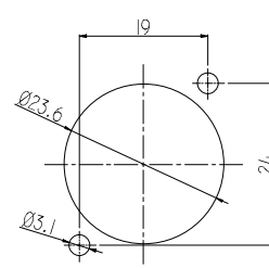
Panel cut out (Rear side)
